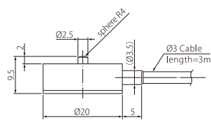
TC-SR(T)□□N/KN-G3
